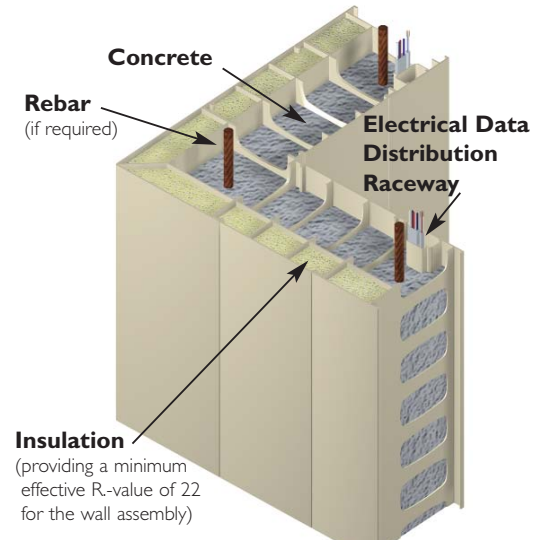
RBS 8i Insulated Wall
